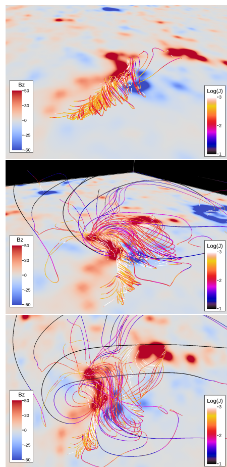
Fig. 6. Illustrations of the field lines above the polarity inversion line for the simulation where \zeta = -175 \text{ km}^2 \text{ s}^{-1} at 10:58 UT on 2017 April 5. The field lines are shown at low (top) and high (middle and bottom) heights above the PIL. The colour coding represents the strength of the electric current, defined as \mathbf{J} = \nabla \times \mathbf{B} along the field lines as given in the right-hand side (Log(J) ranging from 1 to 3). The background image represents the photospheric magnetogram where red represents positive flux and blue negative flux in the range \pm 50 \text{ G} , left-hand sub-panel.
