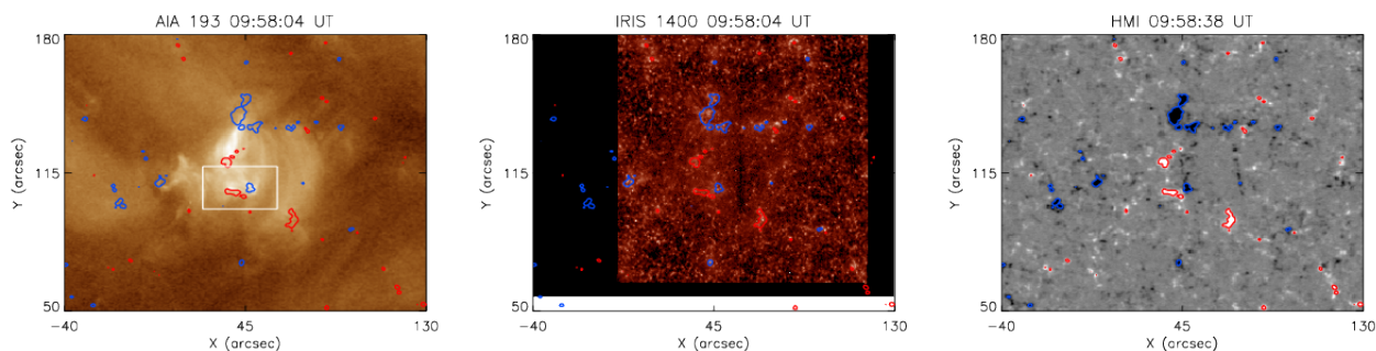
Fig. 1. Small-scale loop system known as a coronal bright point. From left to right: AIA 193 Å, IRIS SJI 1400, and HMI magnetogram images with the CBP in the centre of the field-of-view (FOV). The red and blue contours trace magnetic fluxes at \pm 50 G. The HMI magnetograms are saturated at \pm 50 G. The white-line square in the first panel outlines the FOV shown in Fig. 2.
