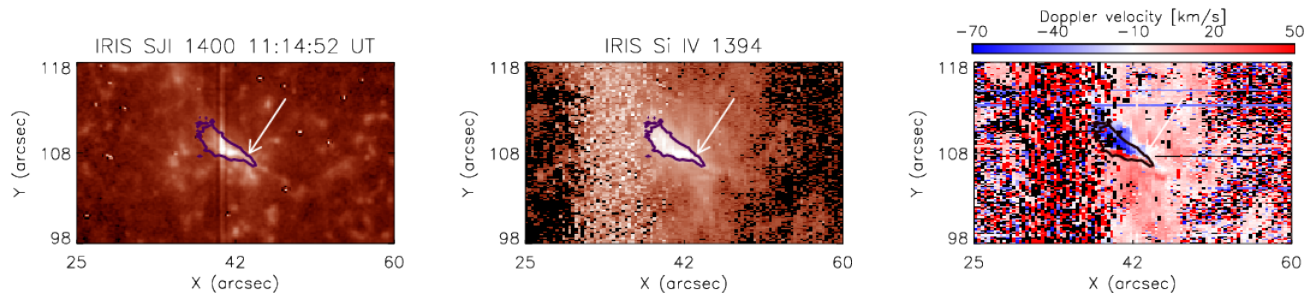
Fig. 4. From left to right: IRIS SJI 1400 image, Si iv 1394 raster intensity and Doppler velocity images. The contour outlines the micro-flare region in the Si iv 1394 raster image that is also overplotted on the SJI 1400 and Doppler-velocity images. The white arrow points at the reconnection site.
