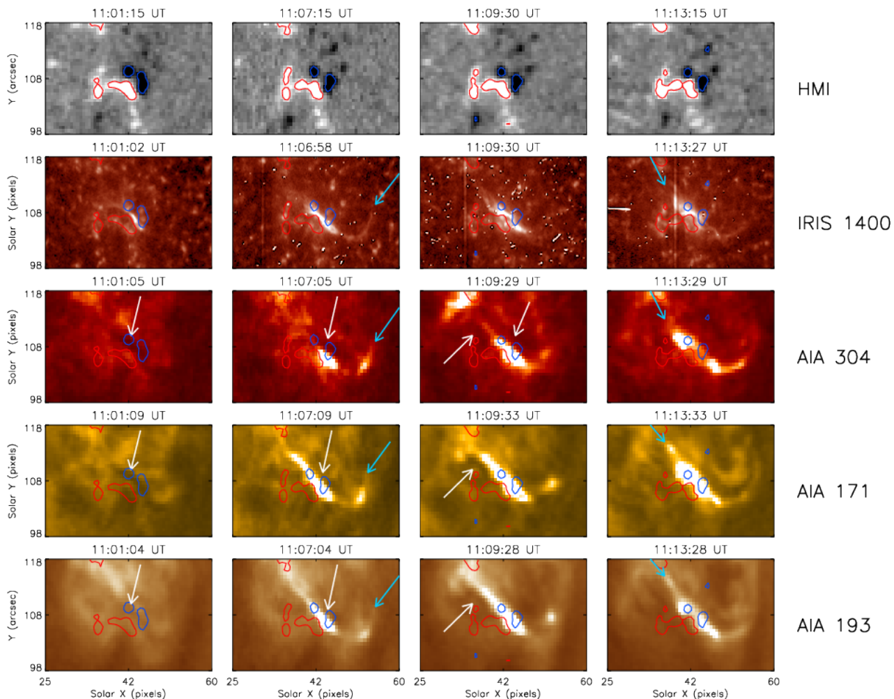
Fig. 2. From top to bottom: HMI magnetograms, IRIS SJI 1400, AIA 304, AIA 171, and AIA 193 images showing the evolution of the eruption. The white arrows point at the mini-filament seen in absorption, i.e. dark feature. The red and blue contours trace magnetic fluxes at \pm 50 G. The cyan arrows indicate the hot plasma up-flows seen as bright extensions from the reconnection site.
