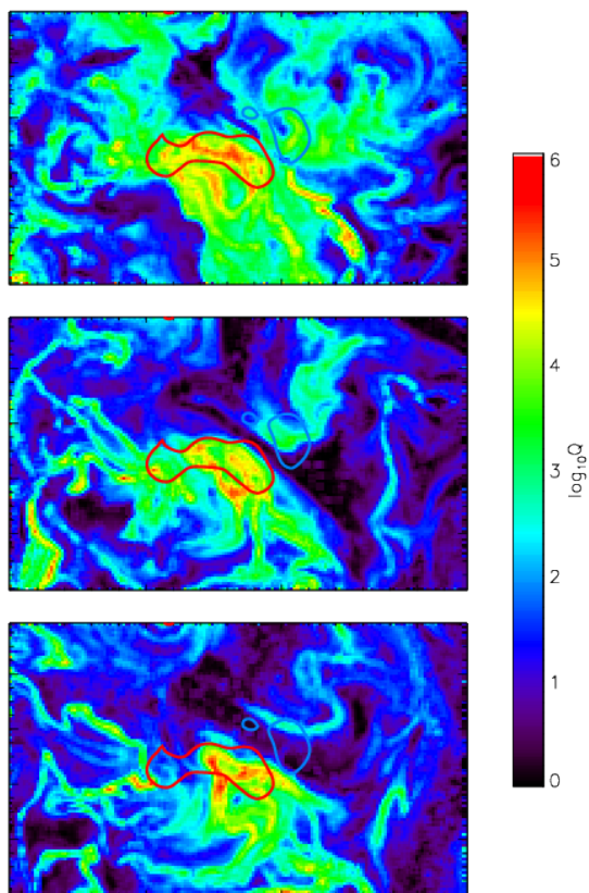
Fig. 7. Three frames showing the spatial distribution of the derived \log_{10}Q values in different horizontal planes above the magnetogram surface. The top panel corresponds to a plane at a height of 110 km, the middle at 1105 km, and the bottom at 2764 km. The blue and red contours denote the negative and positive photospheric magnetic field, respectively at values of B_z = \pm 50 Gauss. The images are smoothed with a boxcar of width 3 \times 3 px 2 .
